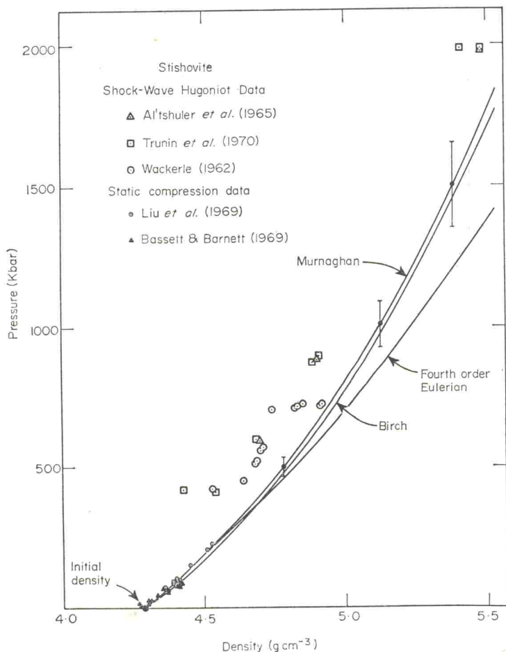
FIG. 1. Pressure-density Hugoniot data for \alpha -quartz and quartzite in the stishovite regime. The calculated isentropes, centred at ambient conditions, are indicated for the present study (Murnaghan), Ahrens et al. (1970) (Birch), and Davies (1972) (Fourth-Order Eulerian).
