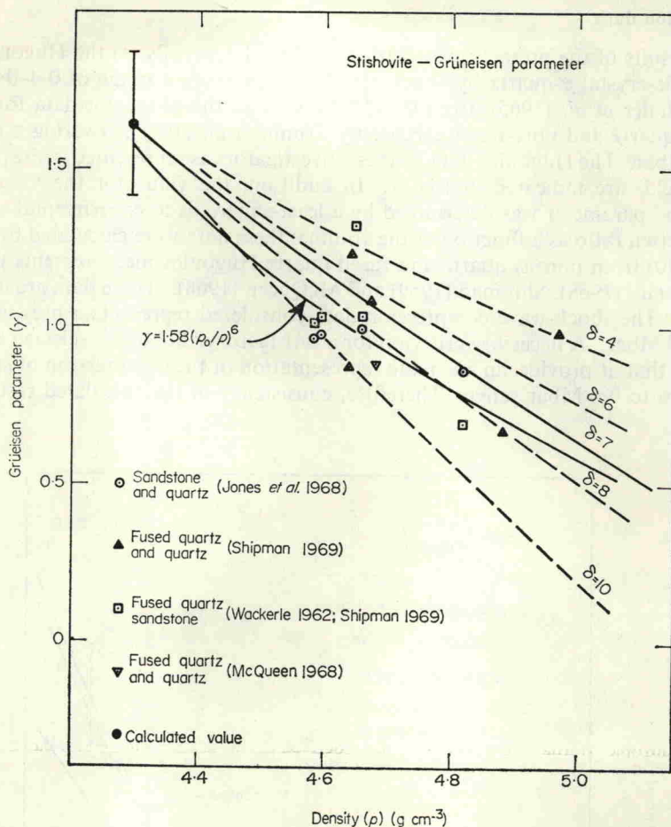
FIG. 2. Grüneisen parameter as a function of density for sandstone, fused-quartz, and \alpha -quartz in the stishovite regime (after Ahrens et al. 1970).
